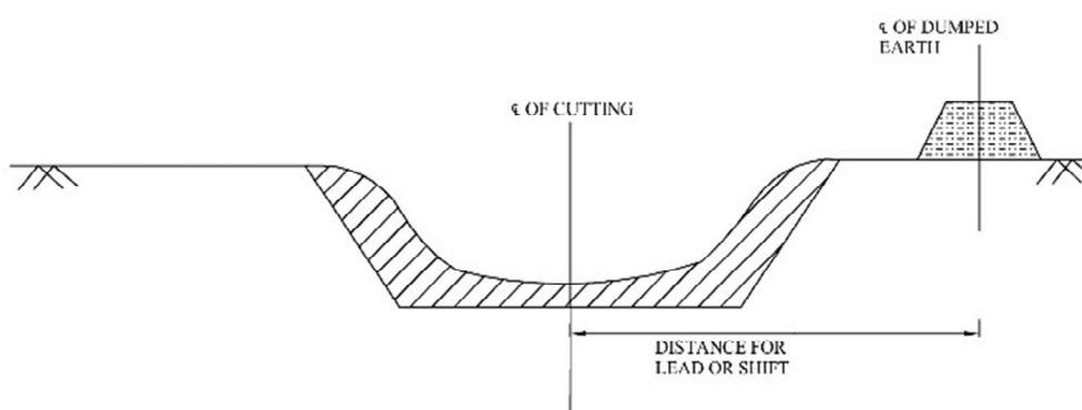
CASE-2: EXCAVATED EARTH DUMPED ON ONE SIDE
