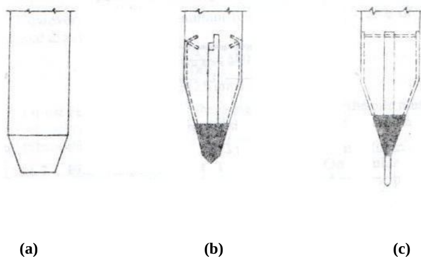
Fig 13.1: Pile shoes
