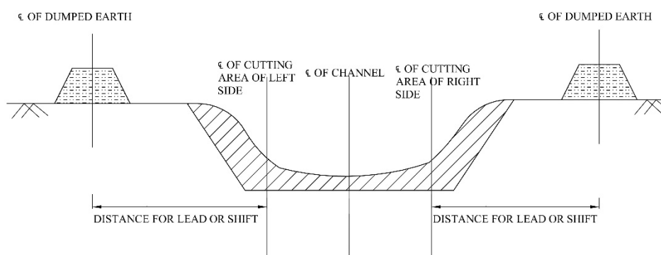
CASE-1: EXCAVATED EARTH DUMPED ON BOTH SIDE
